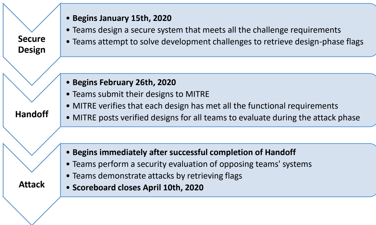
Figure 2. eCTF Phases
