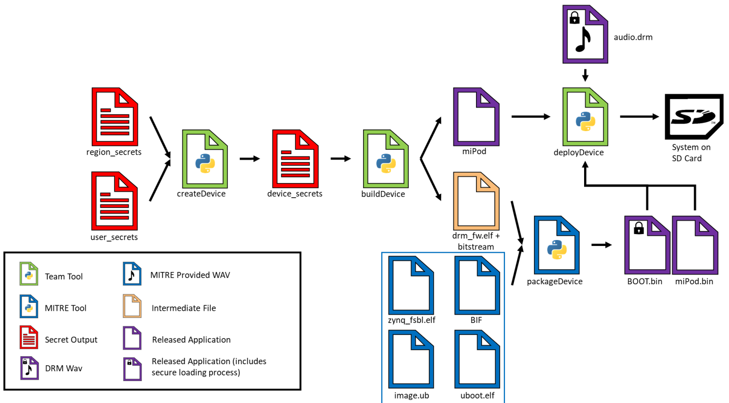
Figure 5: Device Provisioning Process
